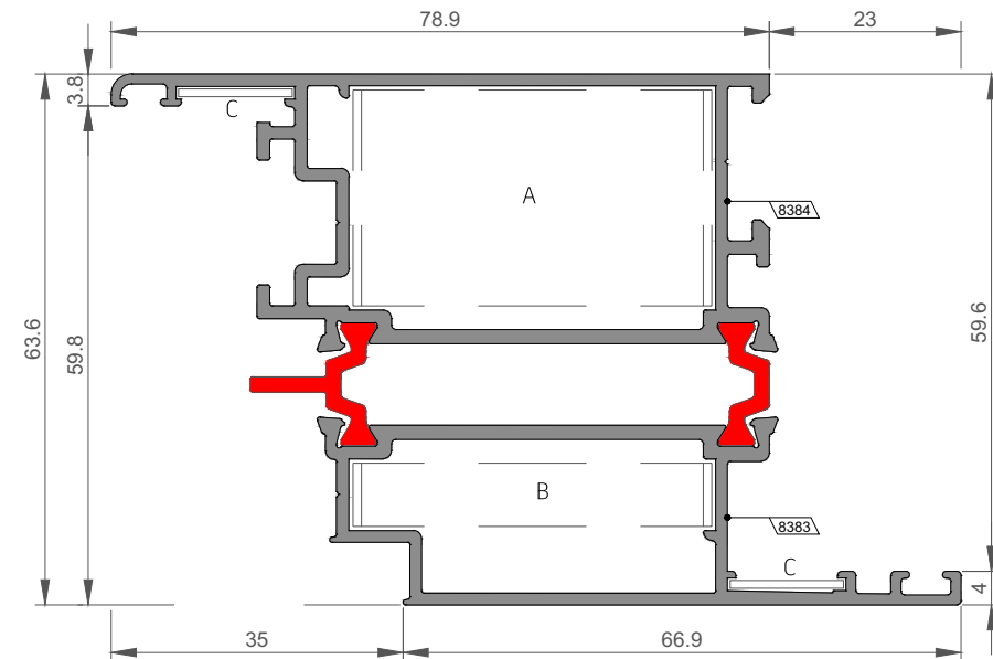
FS-3123 Kanat Profili Sash Profile
