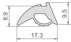
YR-0501014 KAMA FİTİLİ 6.8 mm GLAZING GASKET 99 g/m 160 m - 15 kg
