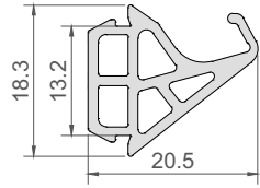
YR-0501004 ORTA BİNİ FİTİLİ CENTRAL STEP GASKET 144 g/m 107 m - 15 kg
