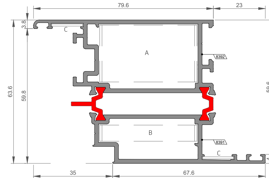
FS-3133 Kanat Profili Sash Profile
